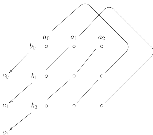
Fig. 1 A schematic depiction of circular convolution. See the text for further detail
