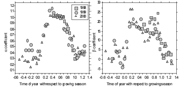
Figure 2: \alpha and \beta coefficients at 10-day intervals over 3 years. Time is fraction through the growing season.
