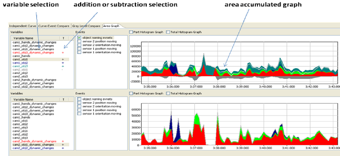
Figure 5. Using area graphs to visualize both an arithmetic combination of multiple data streams and the proportion of each component.
